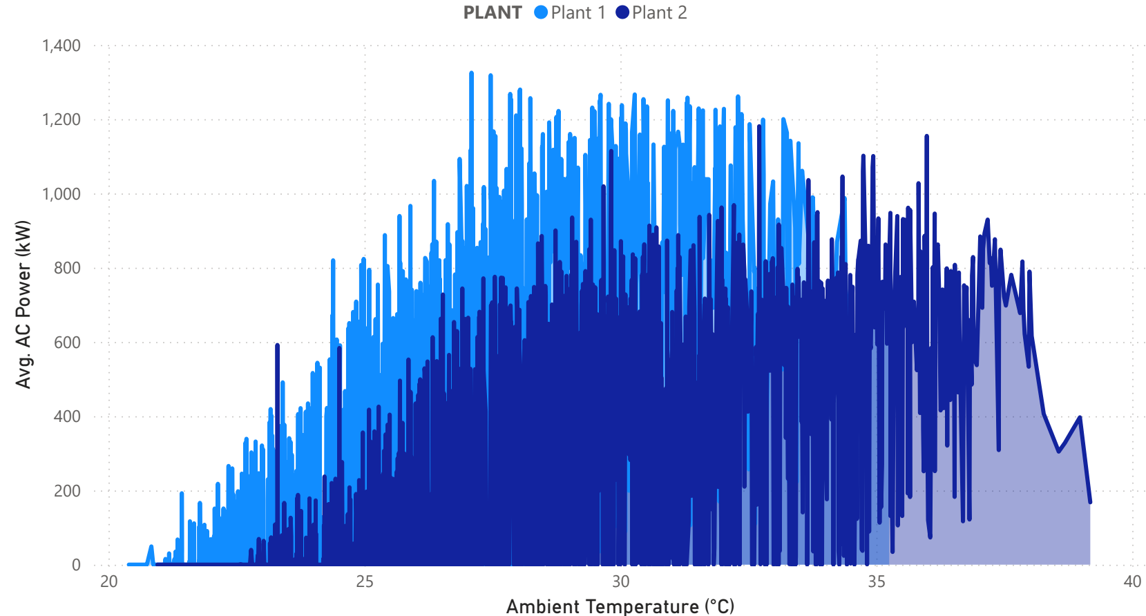
Ambient Temp. vs Avg. AC Power
