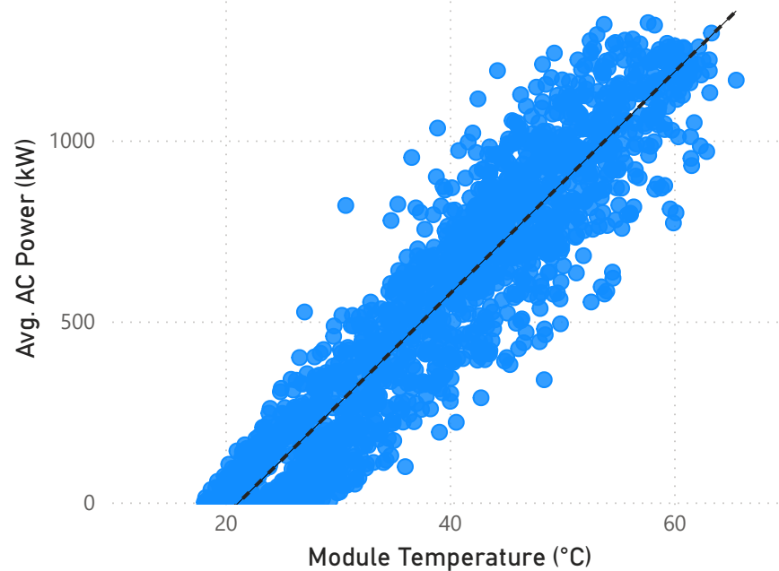
Module Temperature vs AC Power - Plant 2
