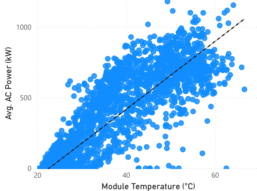
Module Temperature vs AC Power - Plant 2
